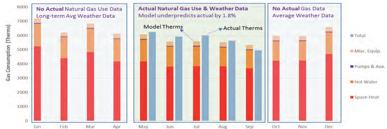
Figure 1b: Natural Gas Consumption - Actual vs Model
